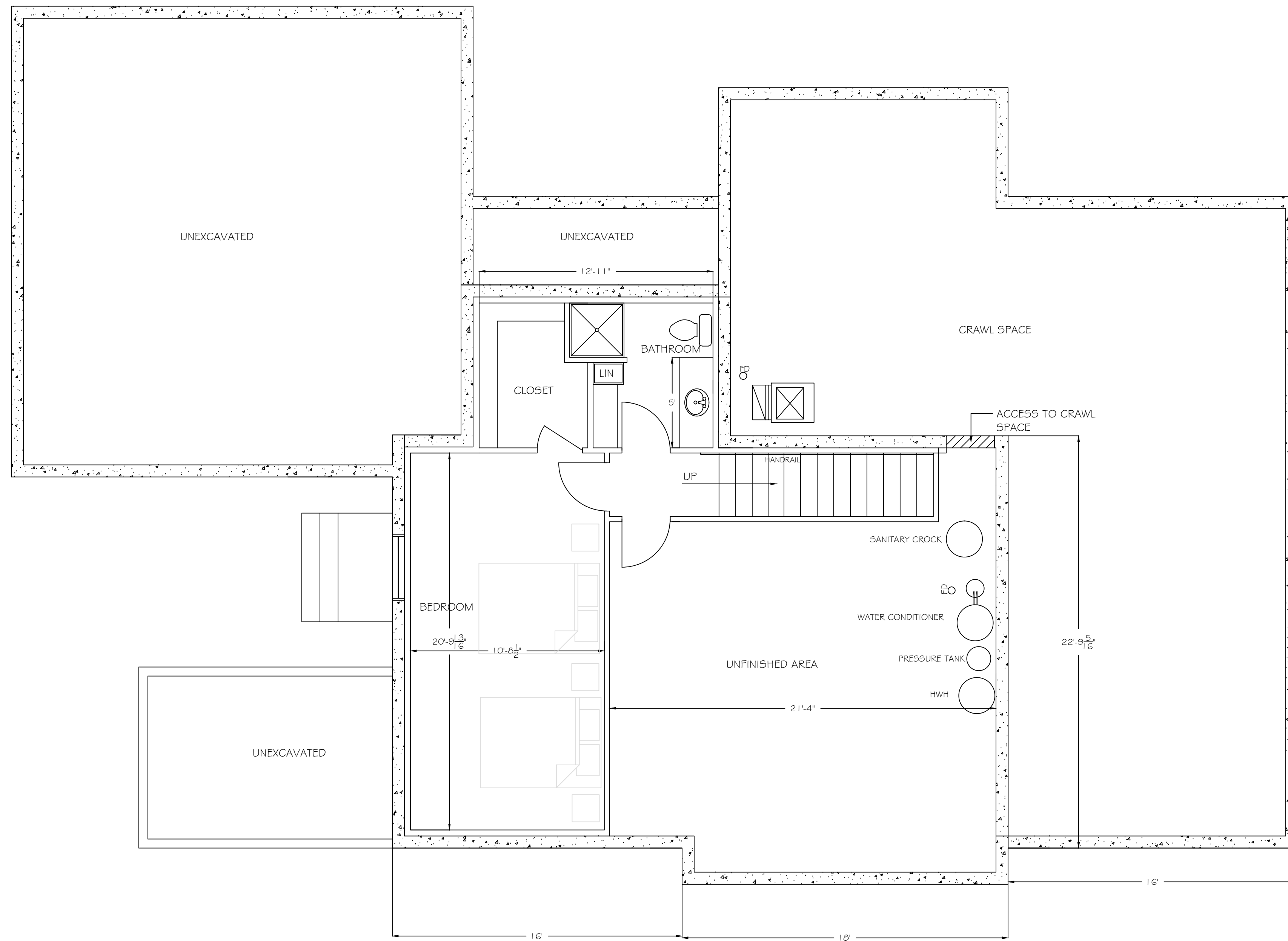
Lower Level Plan Scale: 1/4" = 1'-0"
